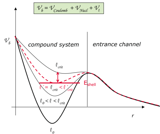
Fig. 1. Schematic illustration of the variation of the fusion potential with \ell and the effect of E_{\text{shell}} .
